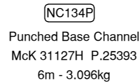
NC134 Base Channel McK 31127 P.25393 6m - 3.096kg
